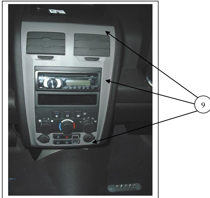
9. Remove gray plastic cover from the center dash panel by pulling out from the bottom.
